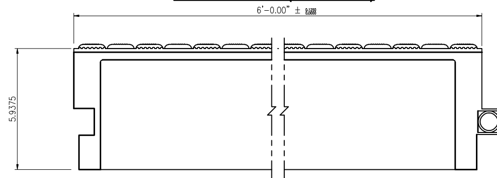
PARTIAL SECTION A-A (SCALE 1:2)
